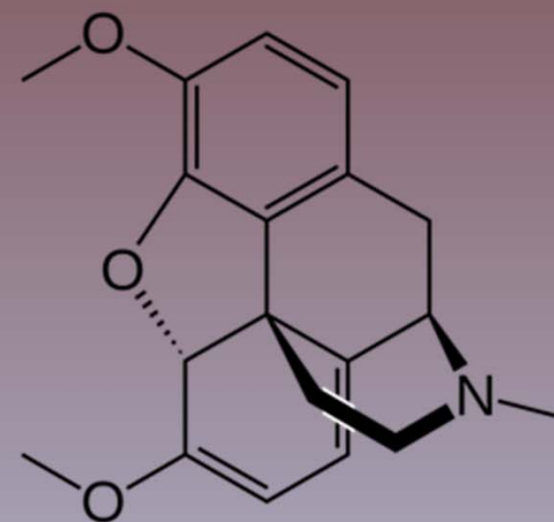
THEBAIN
